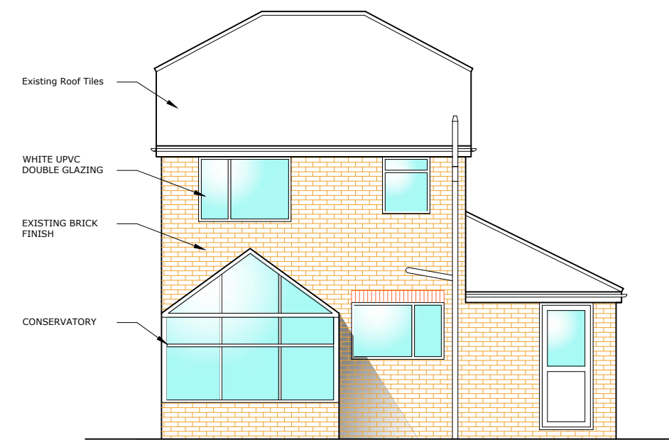
REAR ELEVATION
